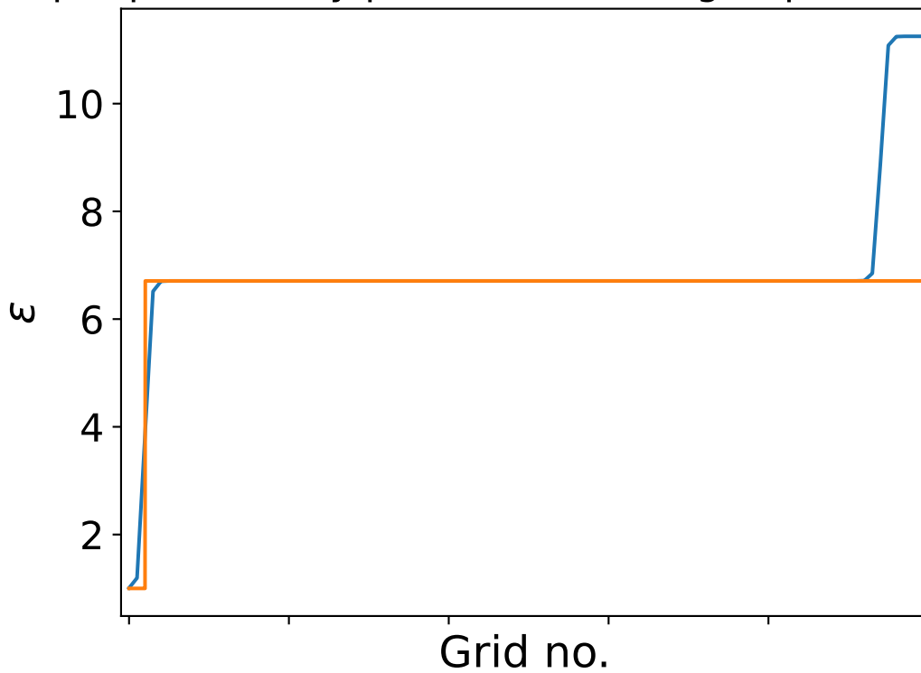
GRCWA permittivity profile. nG = 25, grid points = 100
